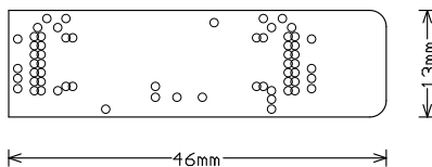
PCB Fabrication Drawing
