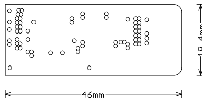
PCB Fabrication Drawing
