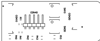
Top Overlay (Top Silkscreen Legend, printed on PCB)
