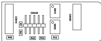
Top Assembly Drawing (Top Assembly Legend, NOT printed on PCB)
