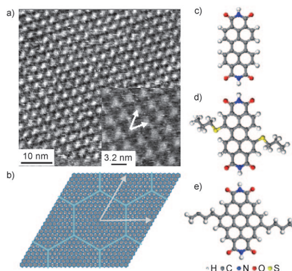
Figure 1. a) STM image of graphene monolayer on Rh(111)/YSZ/Si(111) substrate (sample voltage 1.0 V, tunnel current 200 pA). The periodic features (period 2.95 nm) arise from a moiré pattern because of the mismatch between the graphite and Rh lattice constants. b) Diagram of honeycomb mesh (dark blue) representing graphene overlaid on an array of gray circles representing Rh atoms. The superstructure formed by 12 \times 12 unit cells of graphene overlaid on 11 \times 11 unit cells of Rh gives rise to a long range periodic pattern (unit cell highlighted in light blue) with lattice vectors marked by arrows—these are also identified in the zoomed image shown in the inset to (a). c–e) Structure of the three molecules under investigation: c) PTCDI, d) DP-PTCDI, e) DB-CTCDI.
