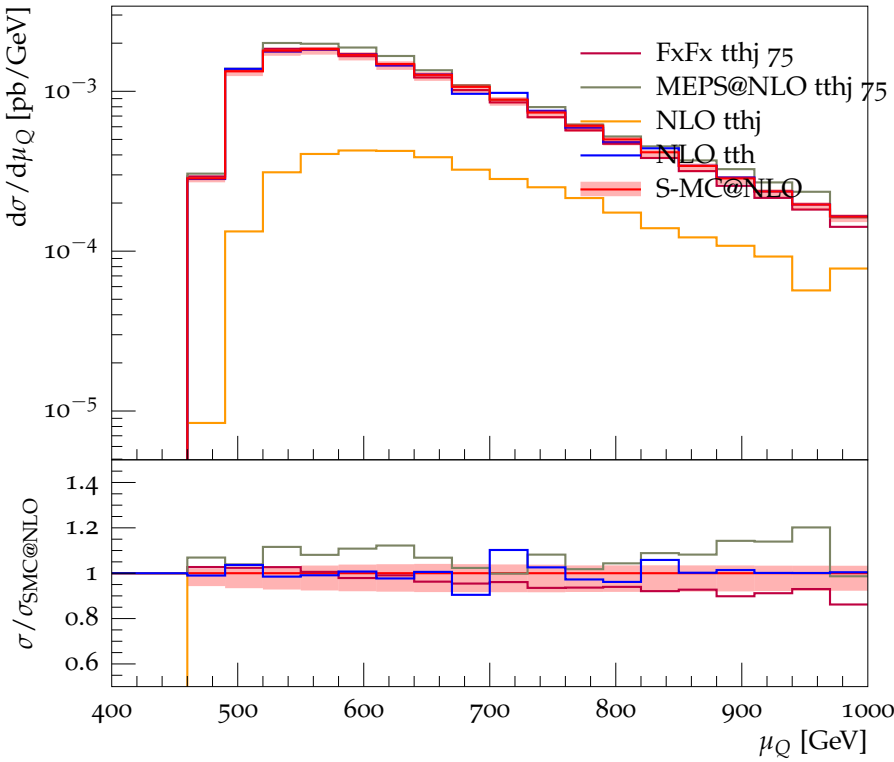
Arithmetic average of t, \bar{t}, H transverse energies ( \mu_Q )
