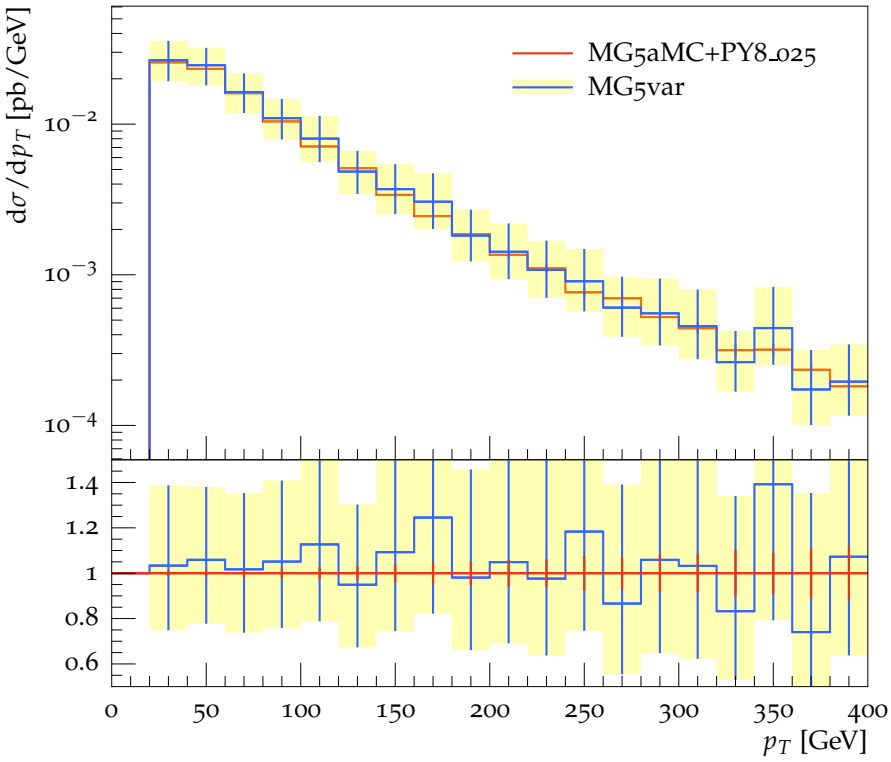
p_T of 1 st light-jet (ttbb cuts)
