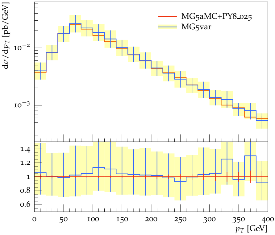
p_T of the 1 st and 2 nd b-jets system (ttbb cuts)
