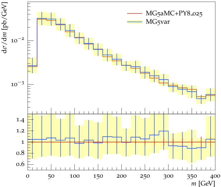
Invariant mass of the 1 st and 2 nd b-jets system (ttbb cuts)
