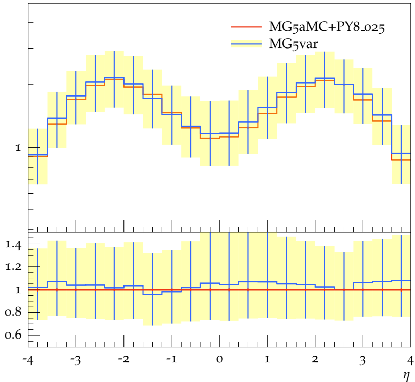
\eta of the t\bar{t} system (ttb cuts)
