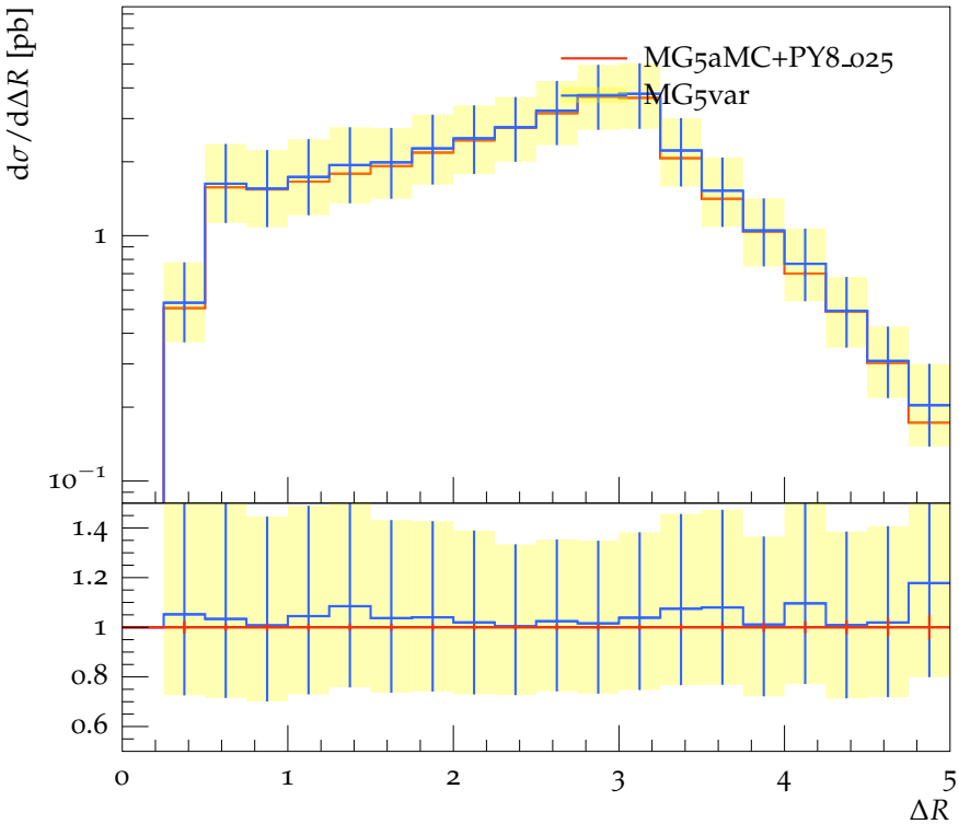
\Delta R of 1 st light-jet and 1 st b-jet (ttb cuts)
