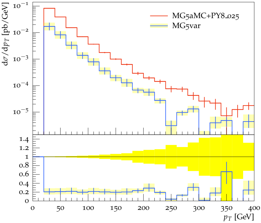
p_T of 2 nd b-jet (ttb cuts)
