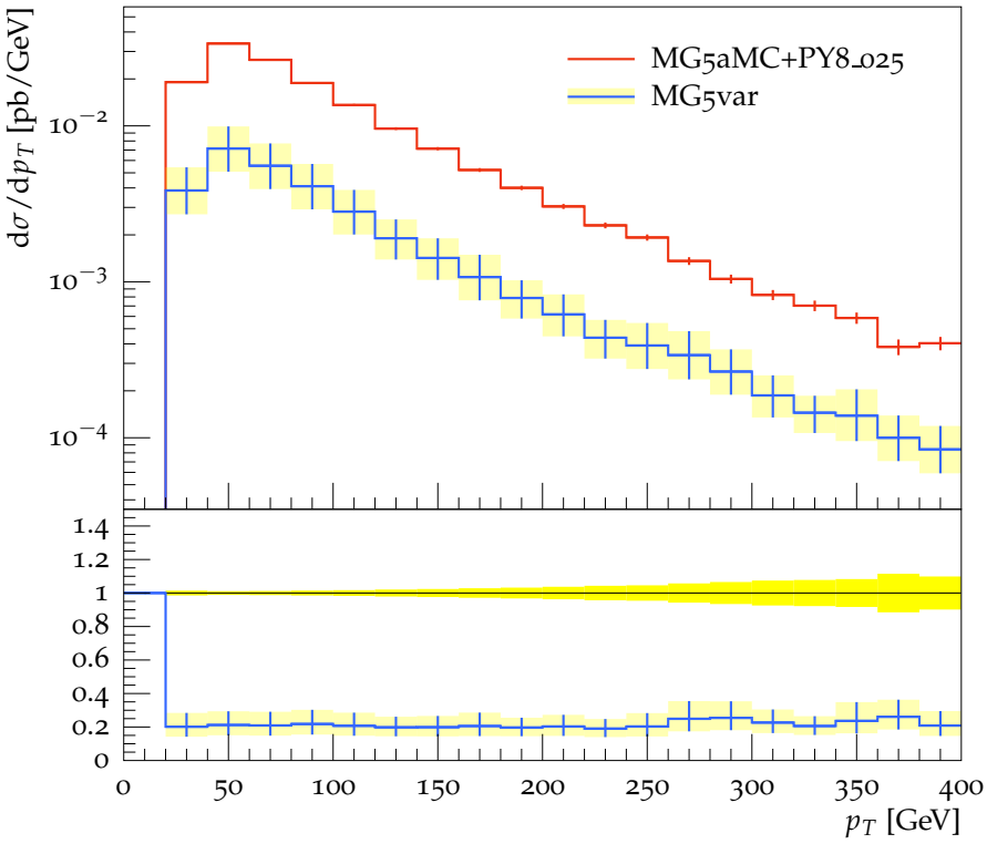
p_T of 1 st b-jet (ttbb cuts)
