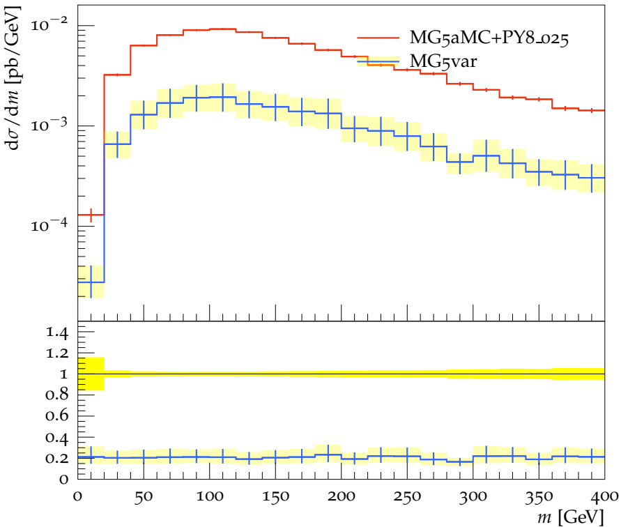
Invariant mass of the 1 st light-jet and 1 st b-jet system (ttbb cuts)
