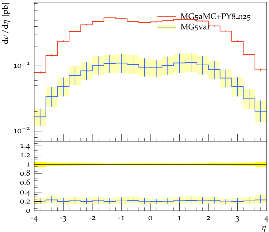
\eta of 2 nd top (ttbb cuts)
