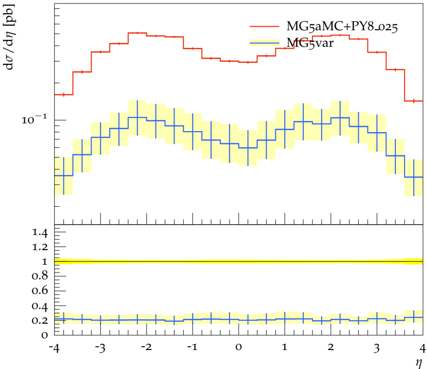
\eta of the t\bar{t} system (ttbb cuts)
