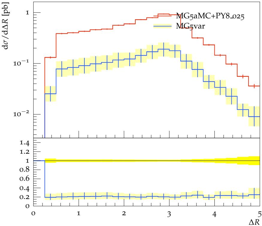
\Delta R of 1 st light-jet and 1 st b-jet (ttbb cuts)
