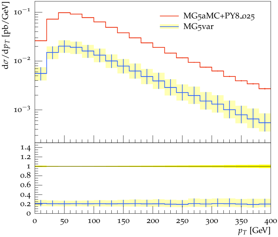
p_T of the t\bar{t} system (ttb cuts)
