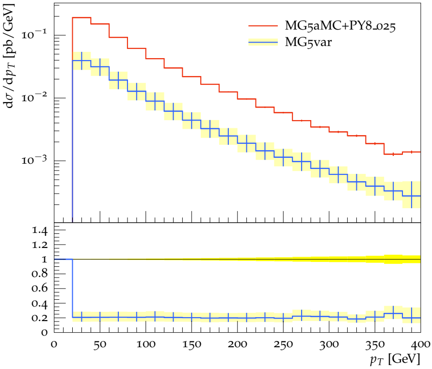
p_T of 1 st b-jet (ttb cuts)
