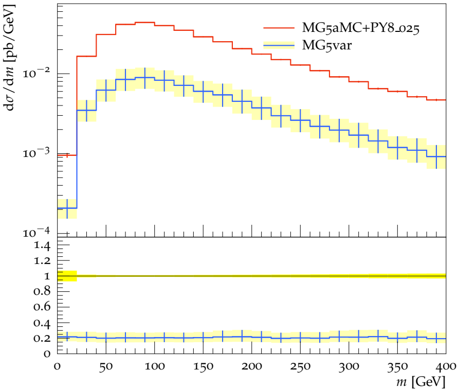
Invariant mass of the 1 st light-jet and 1 st b-jet system (ttb cuts)
