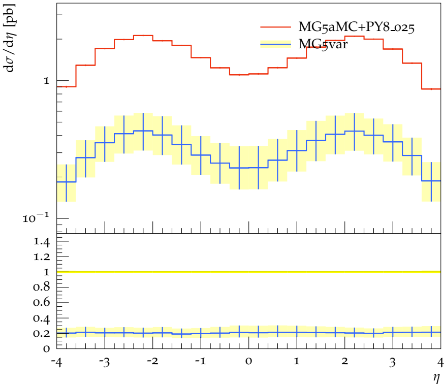
\eta of the t\bar{t} system (ttb cuts)
