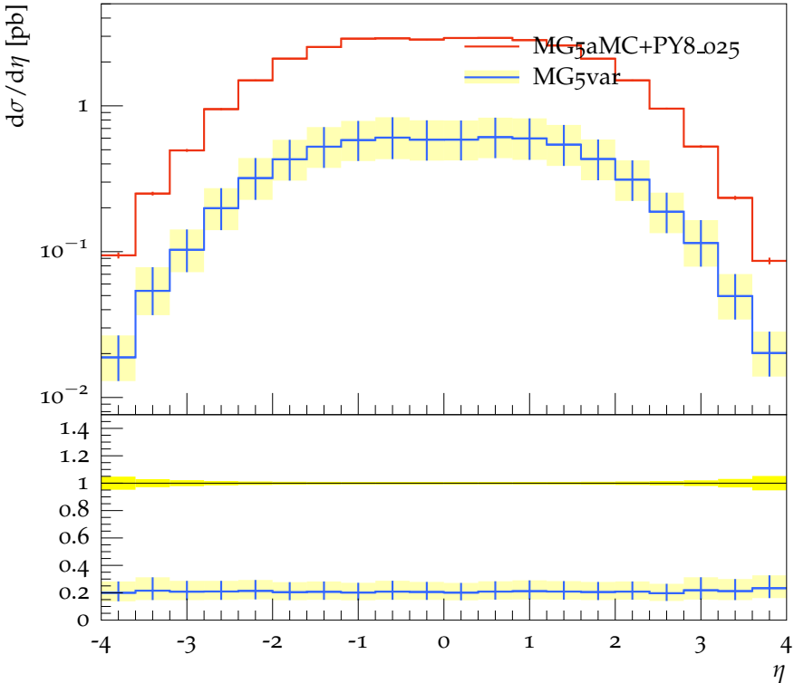
\eta of 1 st top (ttb cuts)
