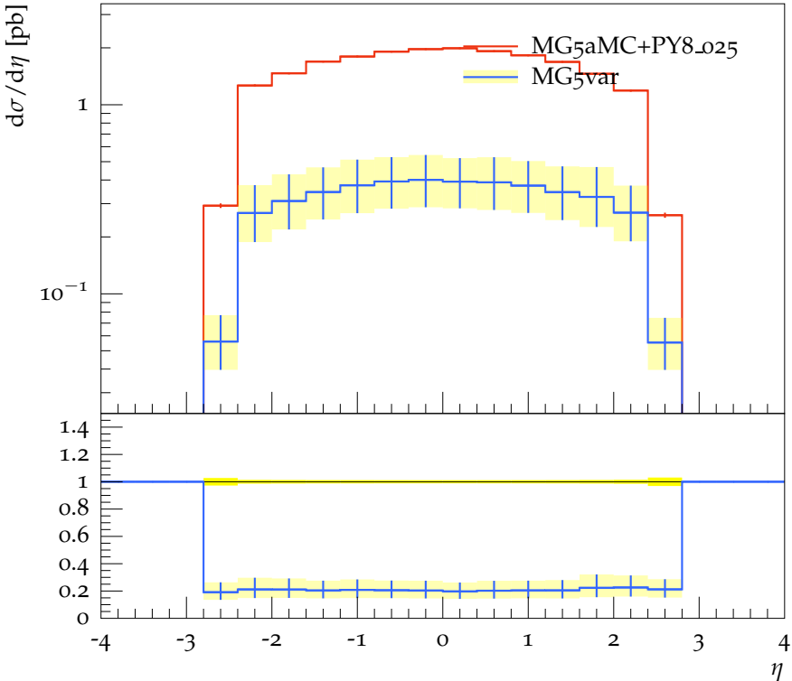
\eta of 1 st light-jet (ttb cuts)
