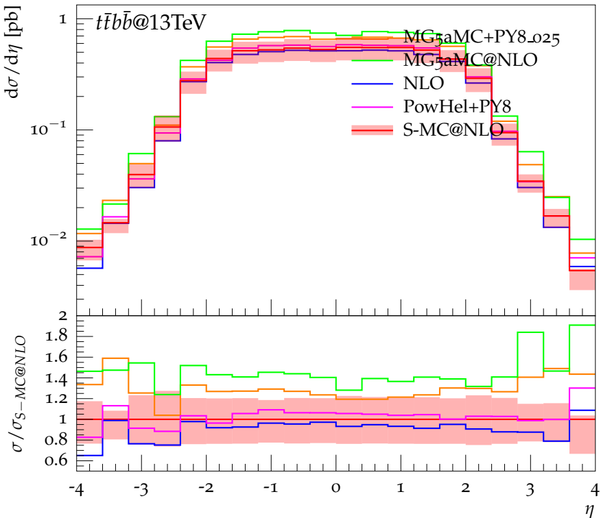
\eta of the 1 st and 2 nd b – jets system (ttbb cuts)
