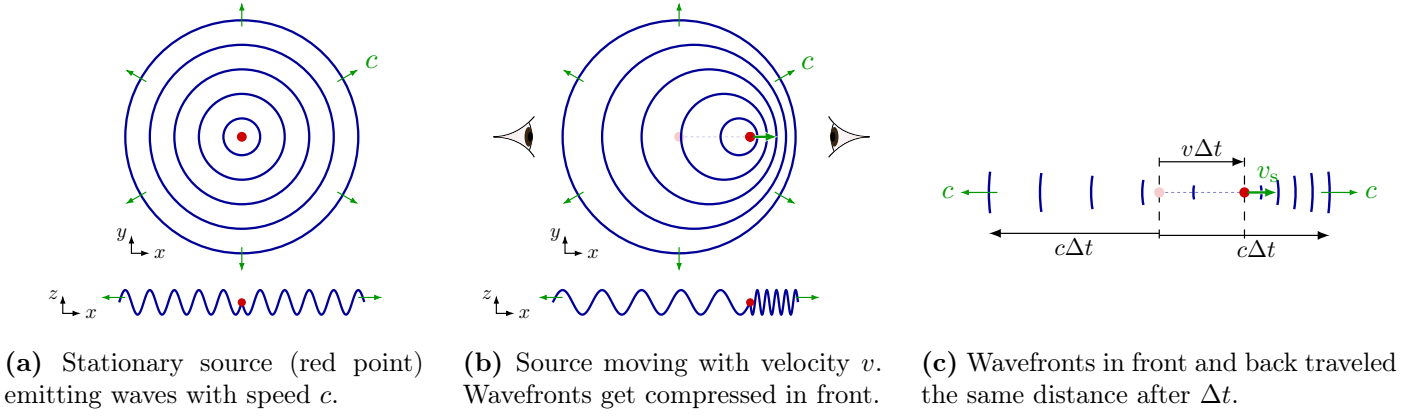
Figure 13.22: Doppler effect in a wavefront diagram: When a source emitting wave moves, the distance between wavefronts (maxima) will vary in each direction.
