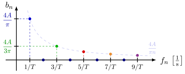
(b) Spectrum of the square wave showing the amplitudes as a function of frequencies f_n = n/T .
