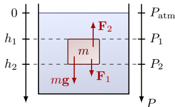
(a) Mass submerged at some depth. The total force due to pressure on the top is \mathbf{F}_1 , and \mathbf{F}_2 on the bottom.
