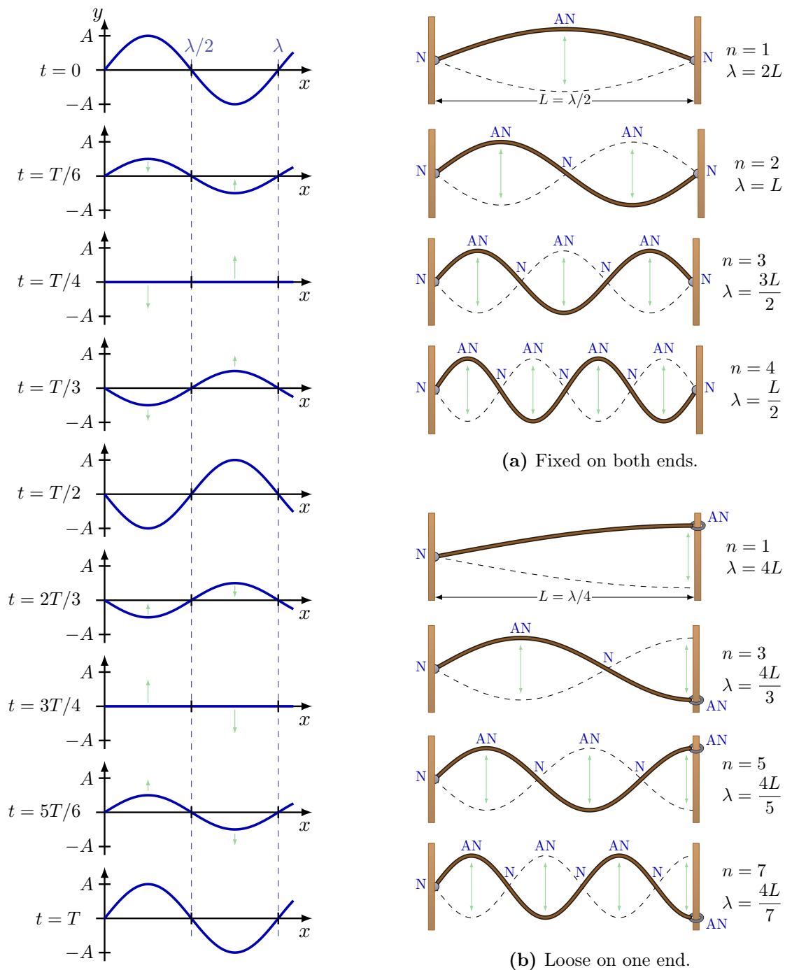
Figure 13.14: Standing wave at different times.
