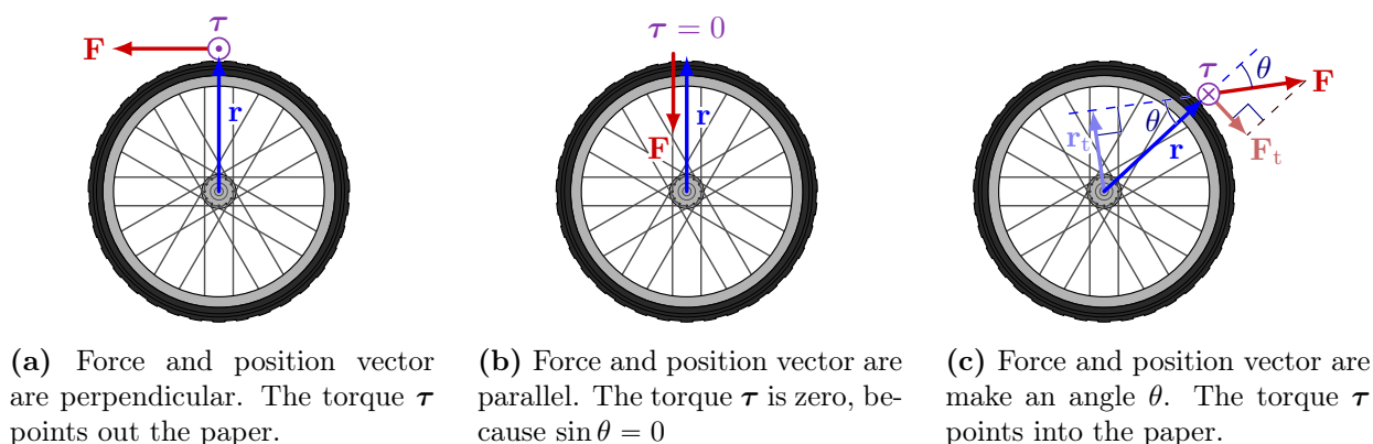
Figure 9.1: Torque \boldsymbol{\tau} = \mathbf{r} \times \mathbf{F} on a bicycle wheel by a force acting on the tyre. The axis of rotation is fixed to the wheel's own axis.
