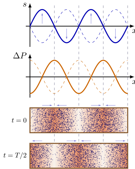
Figure 13.17: Standing wave of harmonic n = 4 in a closed tube filled with air. Top plot shows the local, average displacement s of air molecules in the longitudinal ( x ) direction (blue). The second plot shows the pressure variation \Delta P (orange), which is 90^\circ out of phase with s . The solid line is the wave at t = 0 , while the dashed line is at t = T/2 , when the wave is reversed.
