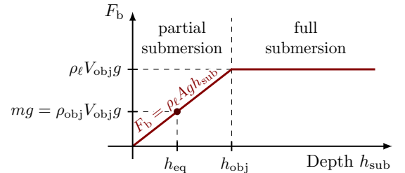
(c) Buoyant force varies with submersion h_{\text{sub}} . Partially submerged, F_b = \rho_\ell A g h_{\text{sub}} . Once fully submerged, the buoyant force is F_b = \rho_\ell V_{\text{obj}}g .
