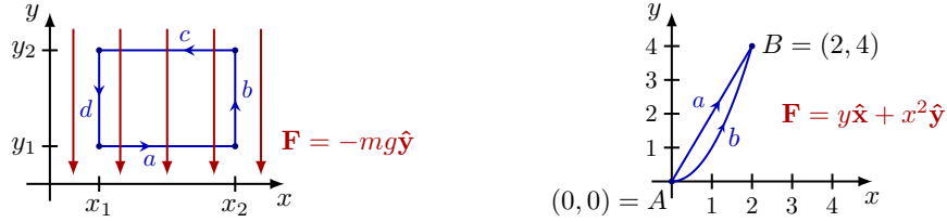
(a) A closed path in a gravitational force field.
