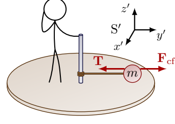
(b) Bob in non-inertial frame S' sees that the mass experiences a centrifugal force creating a tension \mathbf{T} .
