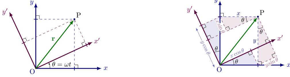
Figure 10.4: Frame S' is rotated counterclockwise with a time-dependent angle \theta = \omega t with respect to frame S .
