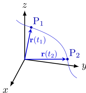
Figure 4.1: Motion of a point in a 3D. The position vector points to different points along the point's path at different times.
