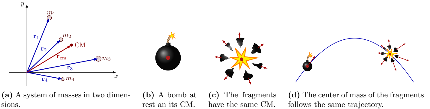
Figure 8.6: Center of mass (red dot) is like the mass-averaged position of a group of masses, or continuous body. If momentum is conserved, the center of mass is constant in space. If there is a non-zero external force, the center of mass will move as if all the mass is concentrated in it and the external force act only on it.
