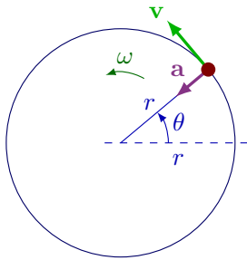
(a) A constant centripetal acceleration is perpendicular to the velocity and changes its direction.
