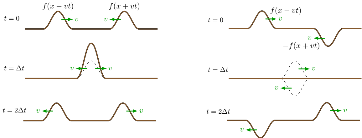
Figure 13.5: Superposition between two oppositely travelling waves in the same medium is a simple linear sum.
