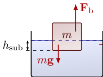
(a) The object is partially submerged and floats if \rho < \rho_\ell , such that F_b \geq mg .
