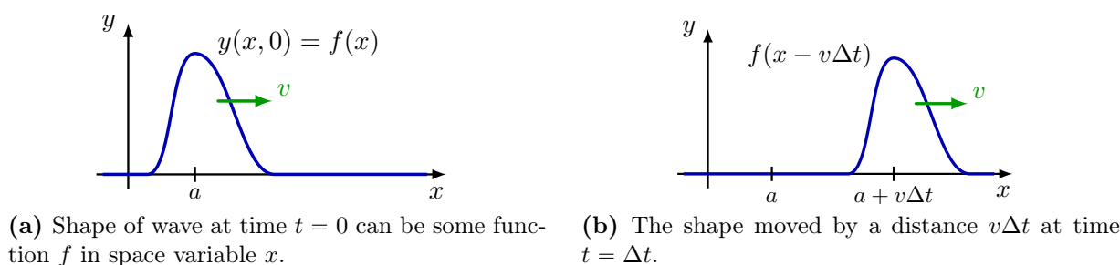
Figure 13.1: A transverse wave is a traveling wave that disturbs a medium in the direction perpendicular to the direction of propagation.
