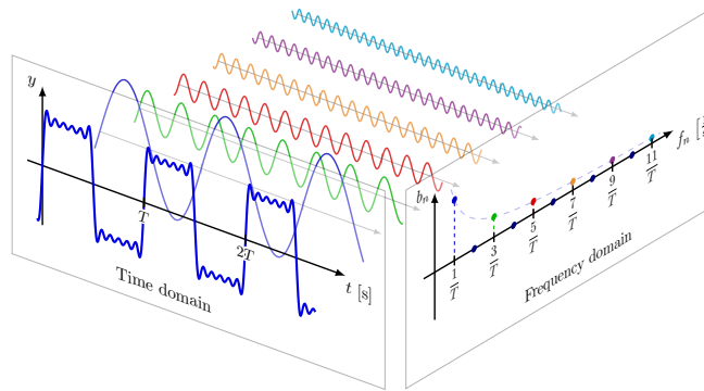
(c) Illustration of Fourier synthesis: Square waves can be approximated by adding up sine waves of frequencies f_n = n/T (i.e. harmonics) with respective amplitudes A_n .
