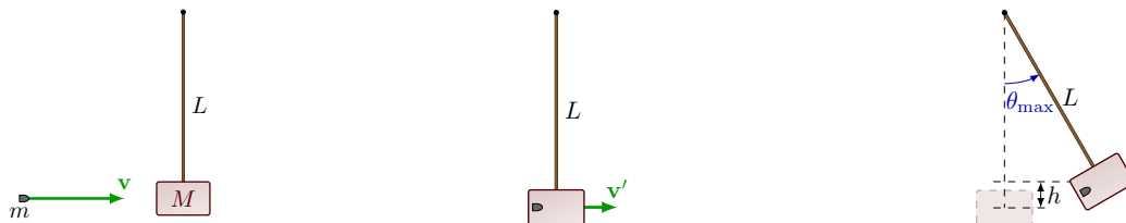
(a) Before: Bullet is shot at a pendulum at rest.
