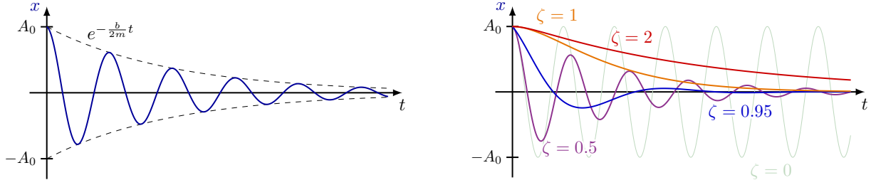
(a) Underdamped oscillation with \zeta < 1 and envelope A(t) = A_0 e^{-bt/2m} .
