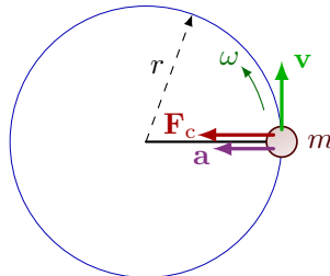
Figure 6.12: A constant centripetal force keeps a mass moving in a circle with constant radius r , angular velocity \omega , and tangential velocity v = r\omega .
