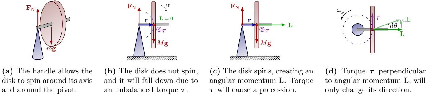
Figure 9.14: A disk with mass M is placed on a pivot with one of its handles. If the disk spins with angular velocity \omega , then it will have an angular momentum \mathbf{L} . A torque will cause the angular momentum to change, leading to the phenomenon known as precession. Precession occurs with angular velocity \omega_p , and the wheel does not fall down.
