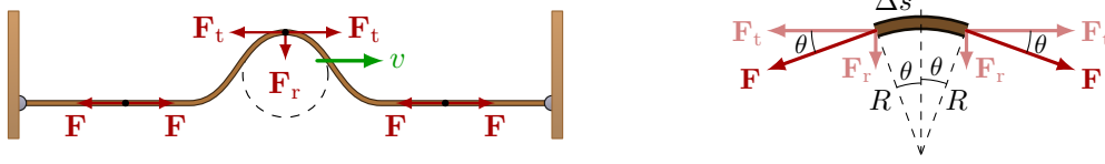
(a) Forces on a string. All across the string, there is a constant tension \mathbf{F} .
