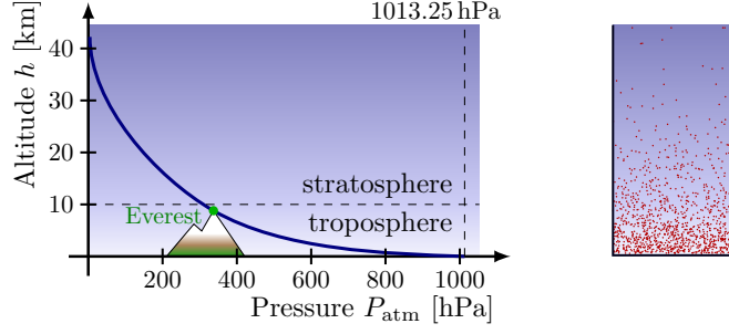
Figure 16.4: The atmospheric pressure varies strongly with altitude. At sea-level, it is typically about P = 1013.25 hPa. Around h = 5.5 km, the pressure is already halved.
