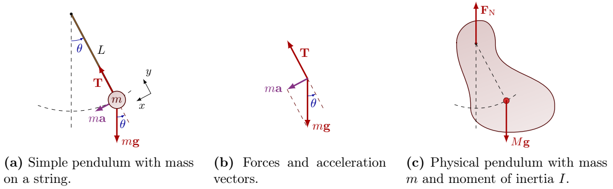
Figure 12.9: A pendulum is a harmonic oscillator.
