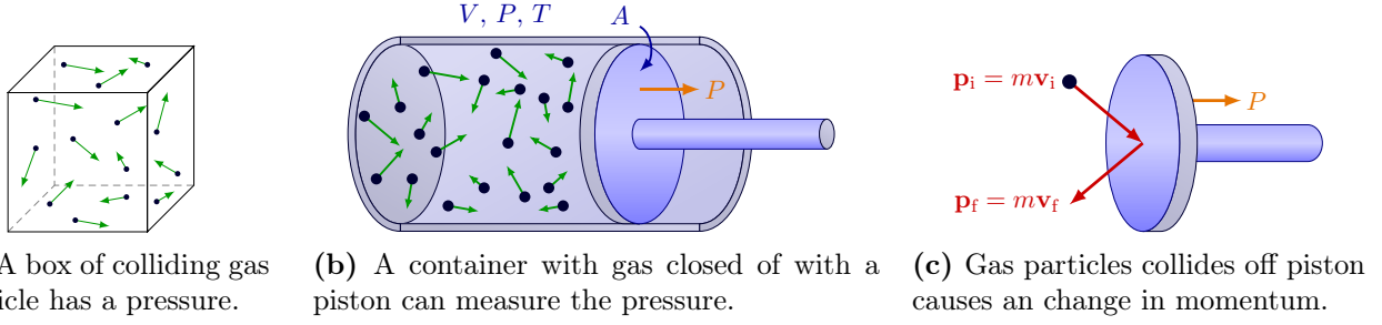
Figure 16.2: Pressure is a macroscopic phenomena caused by collisions of gas particles between each other and on the wall at the microscopic level.
