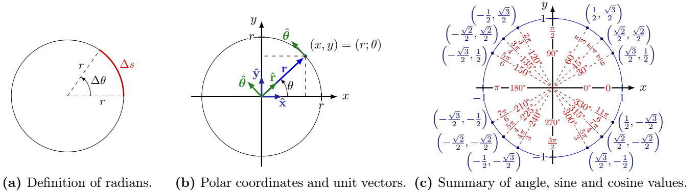
Figure 5.5: Some circle basics.
