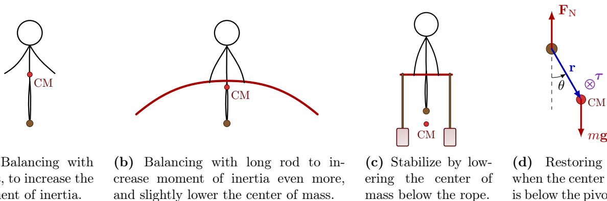
Figure 9.20: Tightrope artist walks on a rope.
