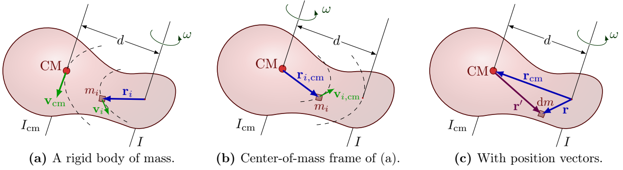
Figure 9.10: Parallel axis theorem: The moment of inertia with respect to an axis parallel to an axis through the center of mass is I = I_{\text{cm}} + Md^2 , where d is the distance between the axes.
