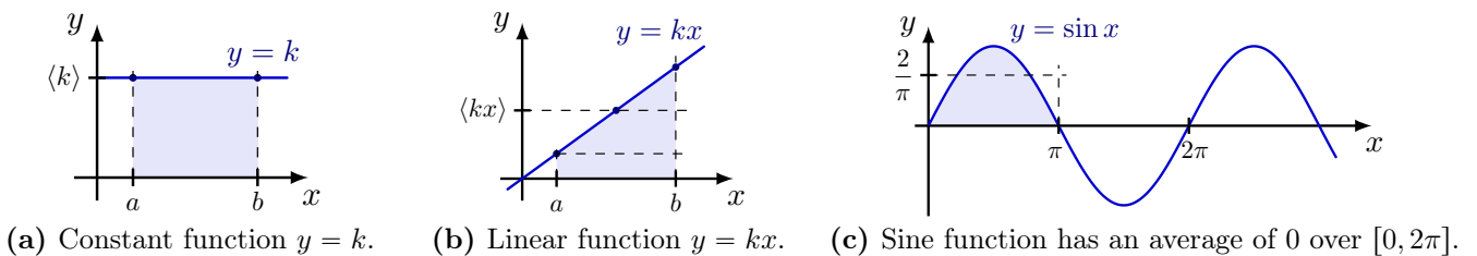
Figure 15.1: Averaging basic functions over some range [a, b] .
