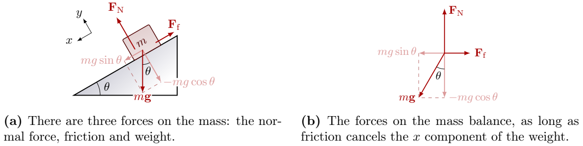
Figure 6.15: Frictional force on a mass on an inclined plane.
