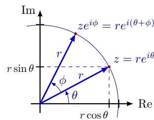
(b) Rotation of a complex number in the complex plane.
