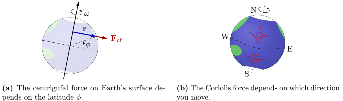
Figure 10.6: Earth rotates, so pseudo forces arise.
