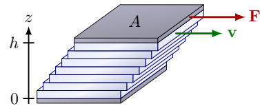
(b) Defining the viscosity \eta by moving the top plate.
