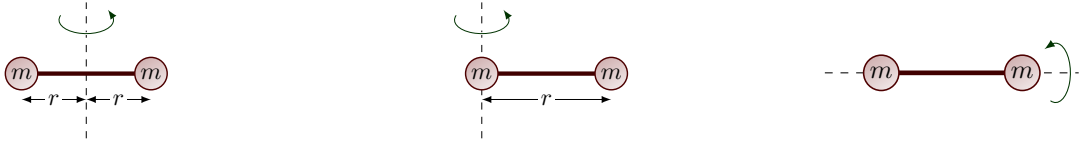
(a) Axis through the middle point between the masses.
