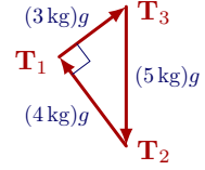
(c) The tensions form a right triangle for 5 : 4 : 3 ratios.
