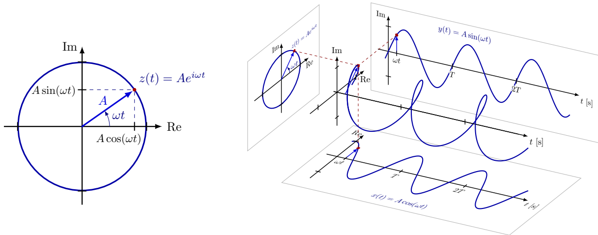
Figure 14.2: A simple harmonic oscillation with amplitude A and angular frequency \omega can be represented by a complex number z = Ae^{i\omega t} .
