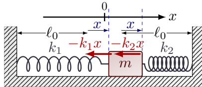
Figure 12.8: Double oscillator: Two springs with constants k_1 and k_2 .
