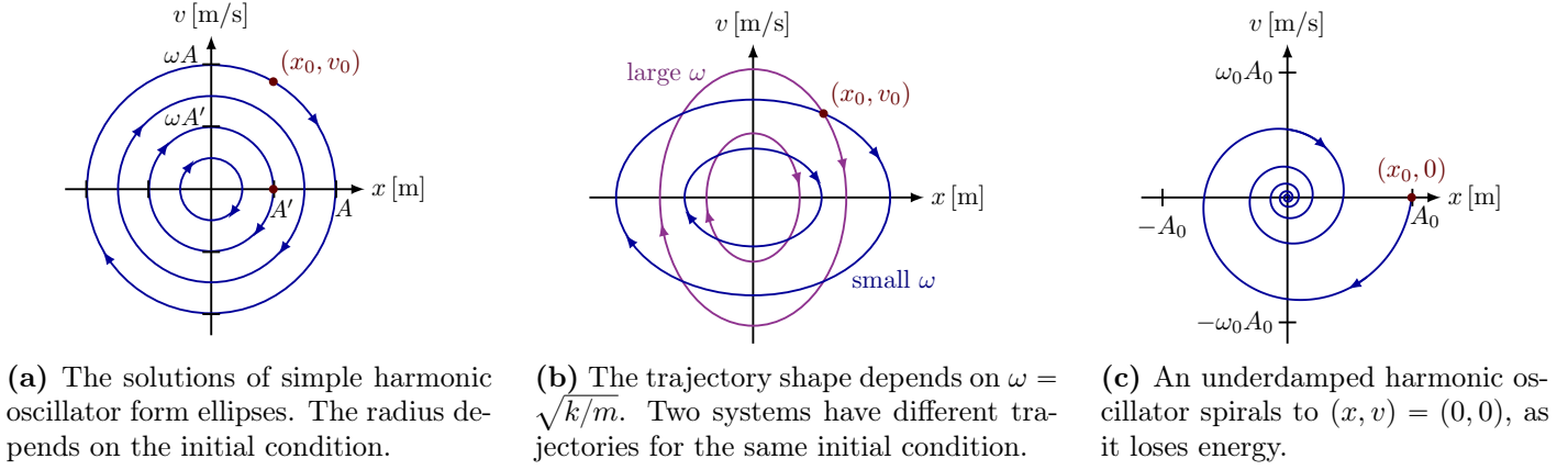
Figure 12.14: Phase portraits for (x, v) of a simple and damped oscillator. The trajectories (solid lines) depends on the system parameters and initial condition (red points).
