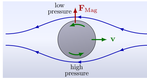
Figure 17.7: A rotating object moving relative to a fluid will feel a difference in pressure, causing a net force \mathbf{F}_{\text{Mag}} .
