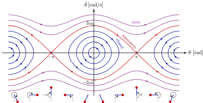
Figure 12.15: The phase portrait of a pendulum with closed (blue) and open trajectories (purple). The edge case where the amplitude is \theta_0 = \pi \text{ rad} and the maximal \dot{\theta} is 2\omega_0 , forms a separatrix (red). Note that because the angle \theta is cyclic; the horizontal axis “wraps” around itself, e.g. any angle \theta is the same point in space as \theta \pm 2\pi \text{ rad} , and therefore corresponds to the same state.
