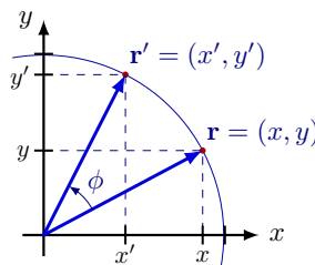
(a) Rotation of a vector in the real plane (See Fig. 10.4).
