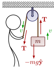
(a) Lifting a mass with help from your body weight. The force is T = mg .
