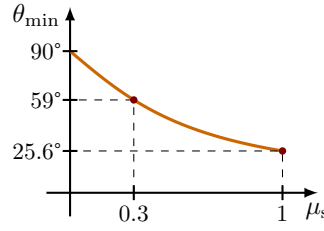
(b) Minimum angle \theta_{\min} as a function of \mu_s (without an person).
