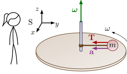
(a) Alice in inertial frame S sees that the mass experiences a centripetal force from tension \mathbf{T} .
