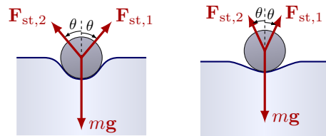
(b) The total surface tension F_{\text{st}} from the points of contact balances the weight of the needle, F_g = mg . The weaker the surface tension, the deeper the indent.
