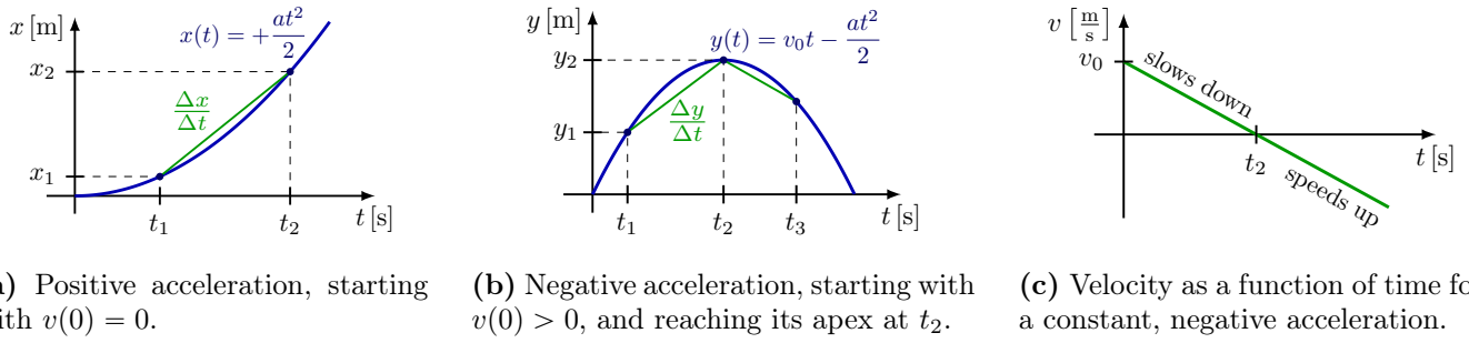
Figure 4.3: Motion in one dimension with changing velocity due to constant acceleration is described by a parabola. The average velocity between two points is given by the slope of the line connecting them (green).
