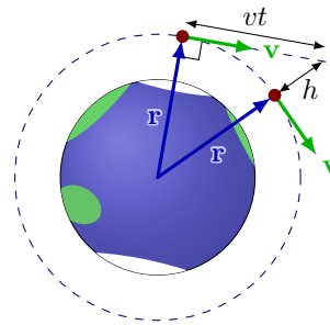
(b) A satellite orbiting the Earth due to gravity creating a centripetal force.
