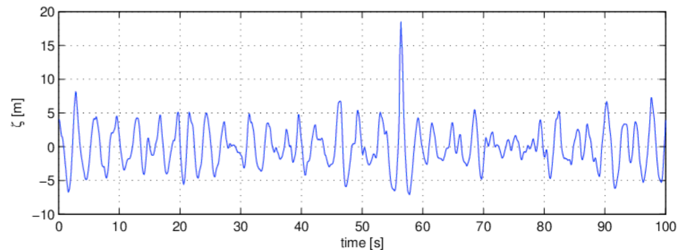
Registration of the New Year Wave-recorded at the Draupner platform in the North Sea on January 1, 1995.
