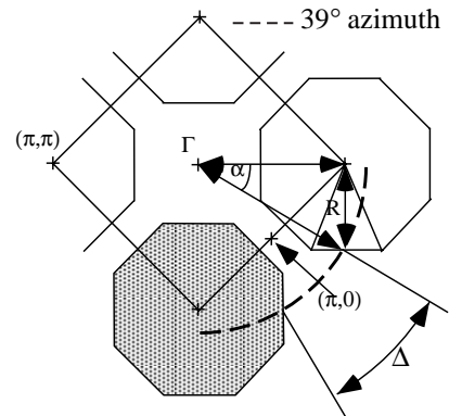
Fig. 4. Approximation of the Fermi surface by regular octagons. The solid square represents the Brillouin zone, the dashed circle segment the location of the 39^\circ azimuthal cut. The Fermi surface intersection angle \Delta is used as a measure for the Fermi surface volume.
